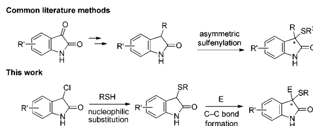
Scheme 1. Preparation of 3-Sulfonyl-3-substituted Oxindoles
